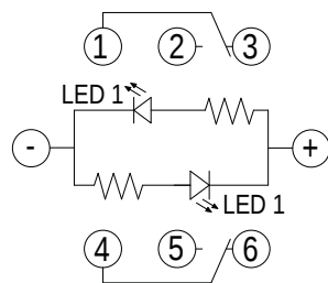
DPDT
